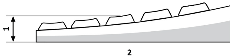
Figure 3-6. Keyboard height measured from the table surface to middle of home row of keyboard. From ISO 9241, part 4 (ISO, 1998). Keyboard height (1) is measured from the horizontal plane (2).
