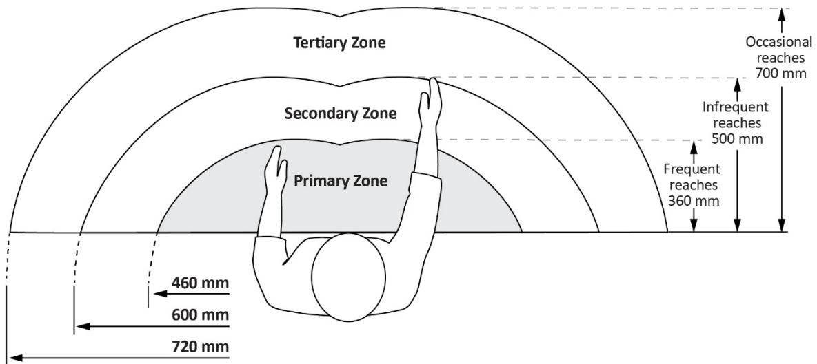
Figure 5-7. Recommended primary, secondary, and tertiary (outside the secondary) horizontal work zones.
