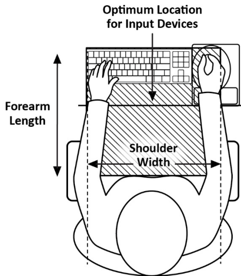
Figure 5-9. Plan view of the recommended space for placement for input devices.
