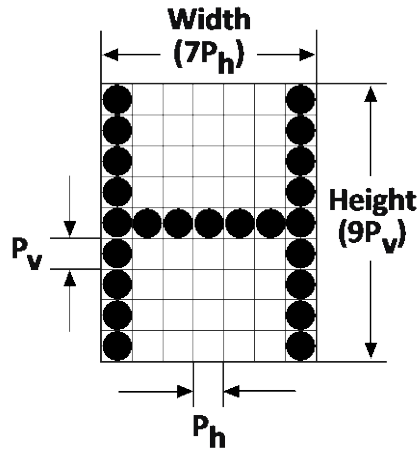
Figure 4-2. Dimensions of characters. The height and width of characters are defined by this figure. Squares represent pixels. P_v and P_h represent the vertical and horizontal dimensions of a pixel, respectively.
