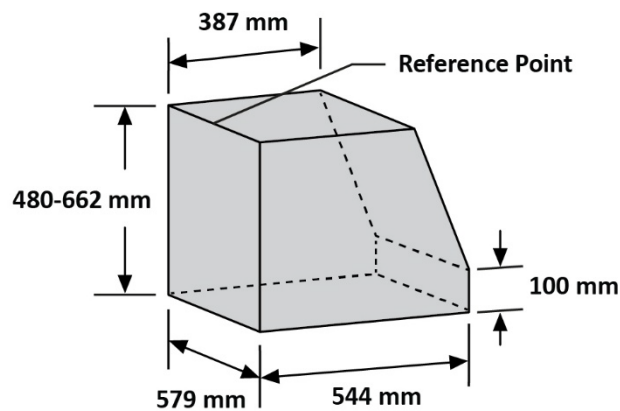
Figure 5-8 Illustration of a side view of the clearance space. The left side faces toward the user.
