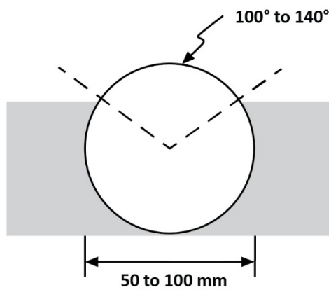
Figure 3-11. Exposed surface and diameter of trackball.
