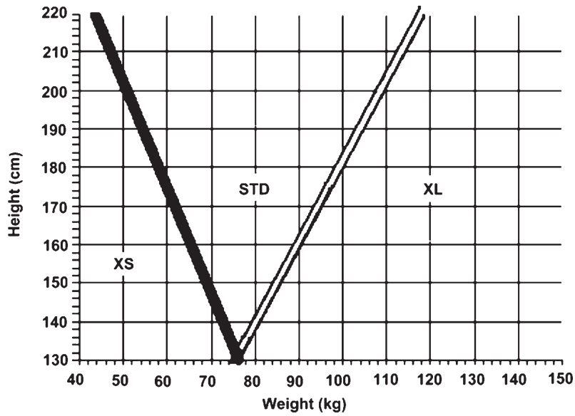
Figure 7. Proposed sizing chart for women for the overhead-style harness in XS and STD sizes (solid line), with an expanded component for the XL size (hollow line; very few women would be expected to use this size) that was derived from combined data for men and women. This model successfully classifies 89.7% of the estimation subset and 94% of the validation subset. The comprehensive logistic regression models, from which this simplified chart was derived, successfully classified 99% of the estimation subset and 100% of the validation subset.
