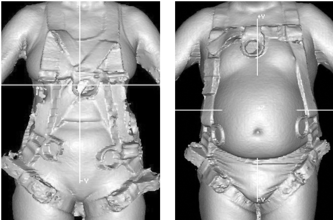
Figure 1. The overhead-style harness (left) and vest-type harness (right) used in the study.
