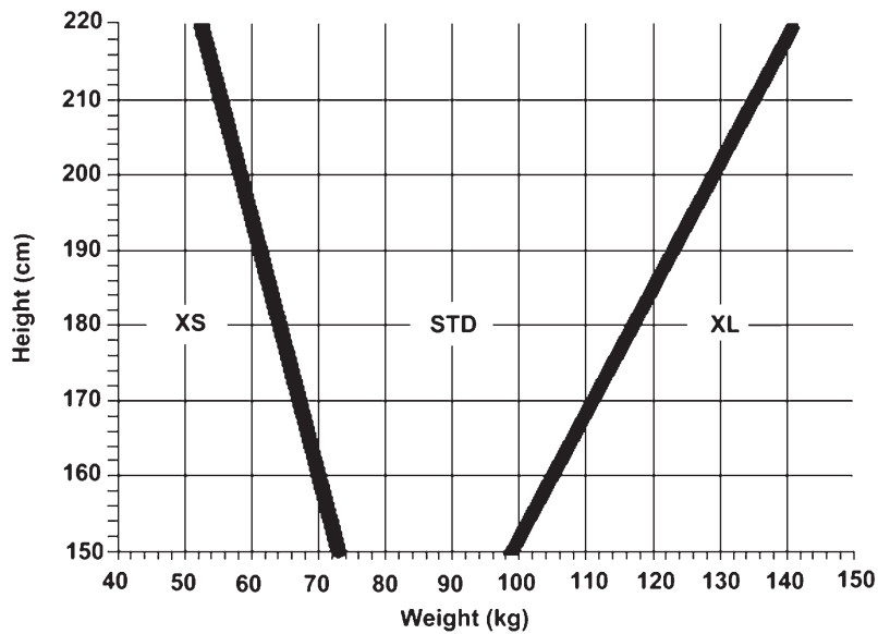
Figure 8. Proposed sizing chart for men for the vest-type harness; this model successfully classifies 96.5% of the estimation subset and 96.4% of the validation subset. The comprehensive logistic regression models, from which this simplified chart was derived, successfully classified 100% of the estimation subset and 95% of the validation subset.
