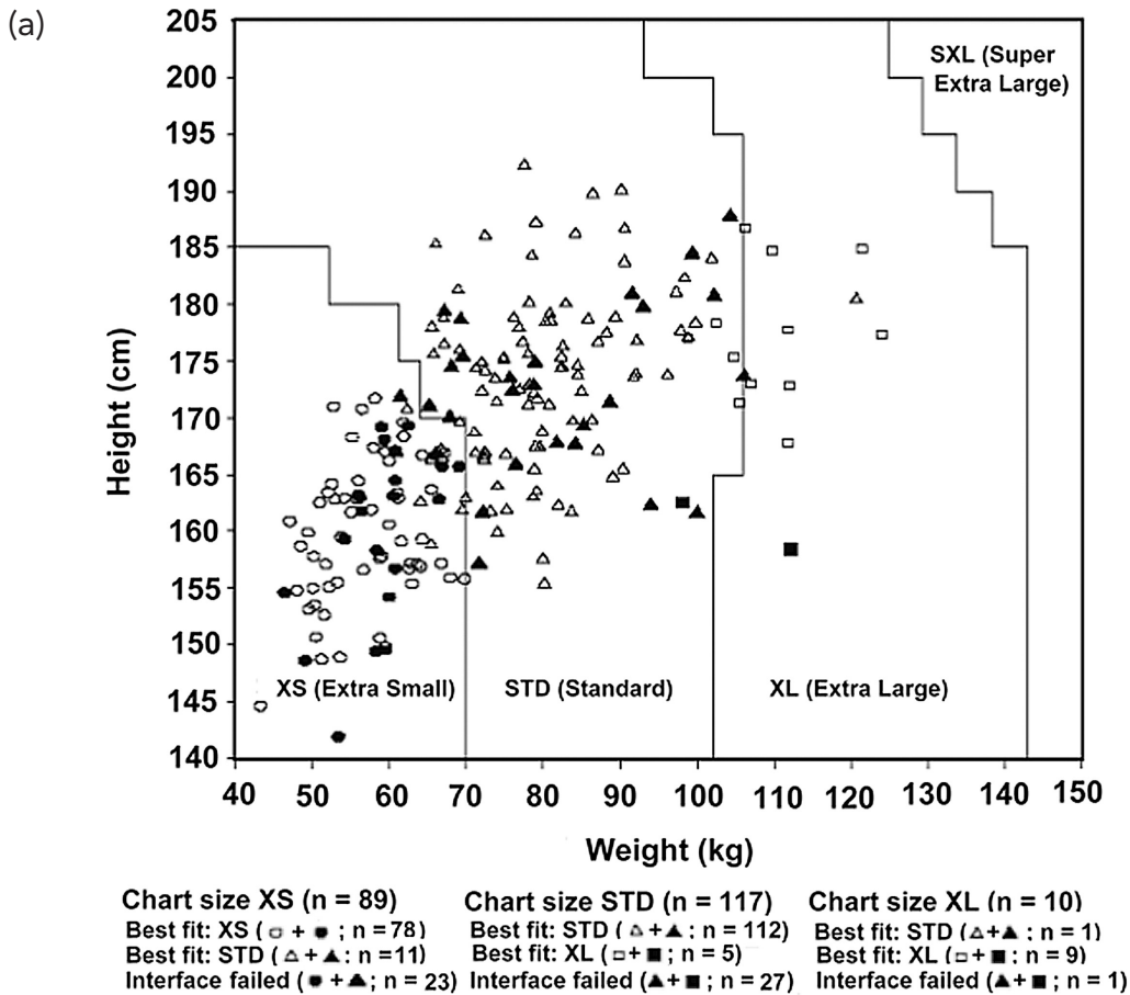
Figure 5. The four divided background areas of these harness size selection charts represent the four sizes of a current harness system based on harness wearers' body weights and body heights for (a) the overhead-style harness and (b) the vest-style harness. Symbols (circles = XS, triangles = STD, squares = XL) represent the best fit sizes. (No
