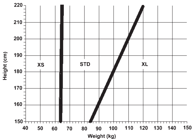
Figure 6. Proposed simplified sizing chart for men for the overhead-style harness. These models successfully classify 97.6% of the estimation subset and 94.3% of the validation subset in this study. The comprehensive logistic regression models, from which this simplified chart was derived, successfully classified 99% of the estimation subset and 100% of the validation subset.
