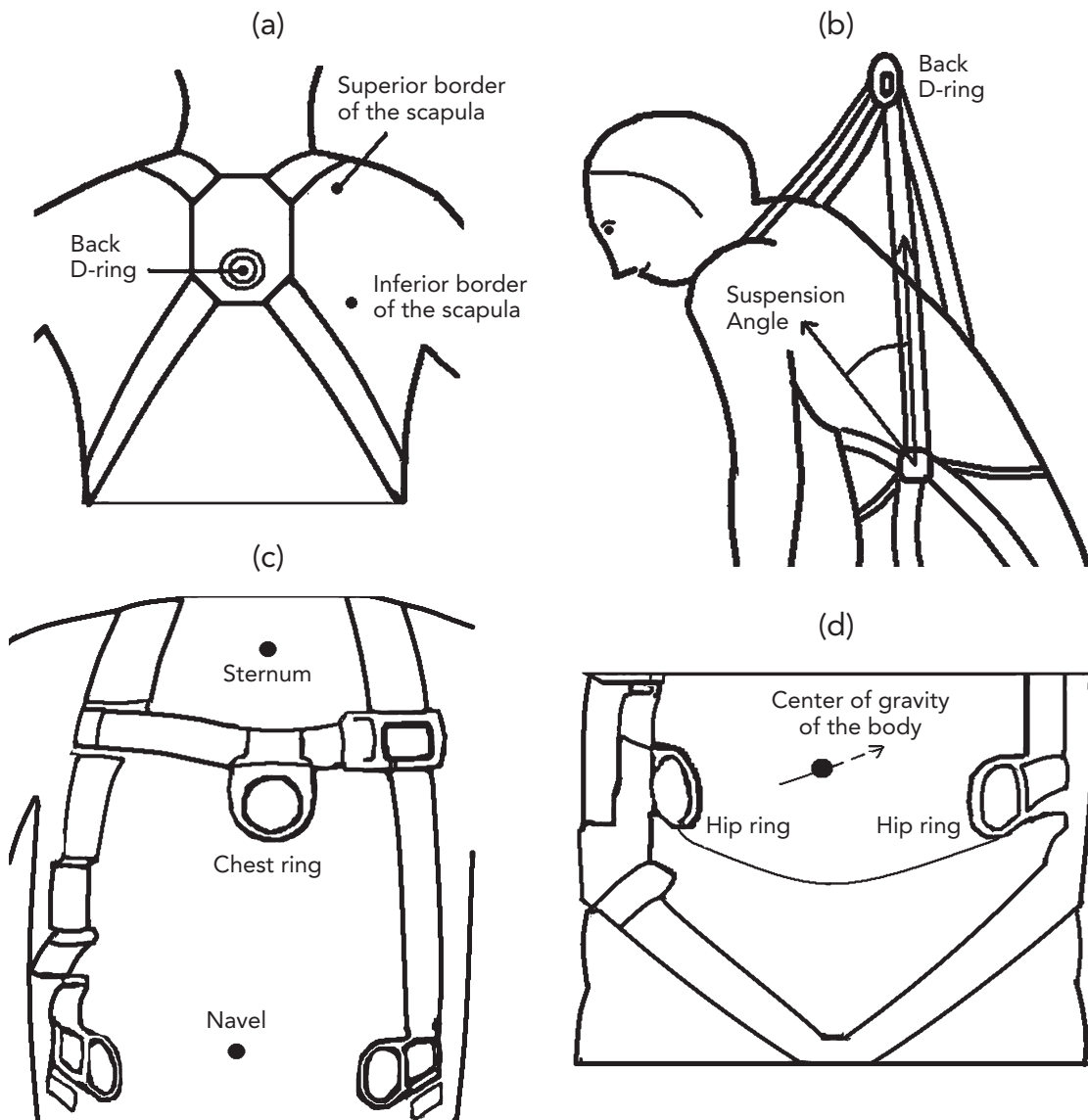
Figure 2. Four criteria – (a) back D ring location, (b) suspension angle, (c) chest ring location, and (d) hip ring location – were used to determine the harness fit score.
